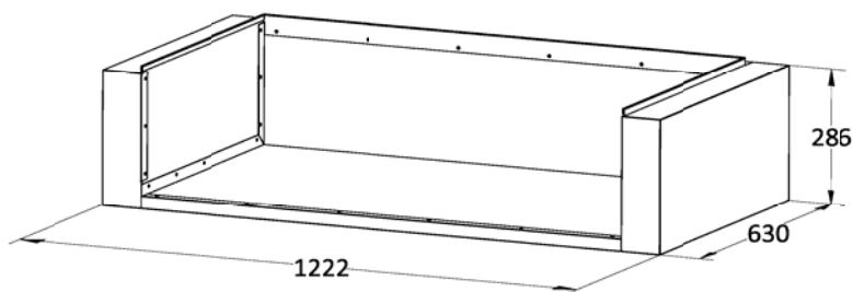
Insulation Jacket/Zero Clearance Box for Deluxe 42 Grill
